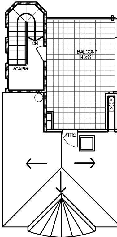
ROOF DECK PLAN
